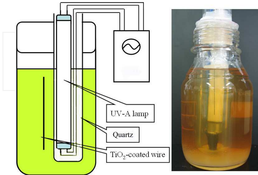
Fig. 2. Apparatus for the assay of anti-adhesion effect of \text{TiO}_2 -coated orthodontic wire.
