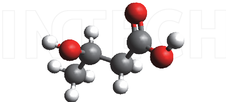
Fig. 5. Schematically illustration of a PHB monomer. The PHB monomer consists of hydroxybutyric acid ( C_4H_6O_2 units) and a methyl group as side chain. Grey = carbon molecule; white = hydrogen molecule, red = oxygen molecule.
