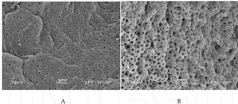
Fig. 5. Scanning electron micrographs of sound (A) and carious (B) human dentin after irradiation with a Er,Cr:YSGG laser ( \lambda = 2078 nm, pulsed width of 140 \mu\text{s} , repetition rate of 20 Hz, beam diameter of 750 \mu\text{m} ). A - As sound dentin is irradiated by Er,Cr:YSGG laser an irregular dentinal surface is created by the ablation process. Dentinal tubules are open and peritubular dentine can be easily detected around all dentinal tubules; B - Carious irradiated dentin still presents open dentinal tubules, but are larger in diameter and filled with debris from the carious tissue. Note that these features are completely distinct from the irradiation by Er:YAG laser. Original magnification: 1000 X.
