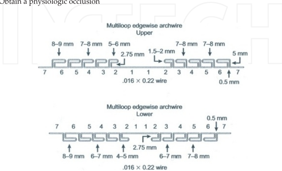
Figure 3. The MEAW's are constructed with .016x.022 stainless steel (bracket 0.018 – inch slot) or .017x.025 ss (bracket 0.022 – inch slot).
